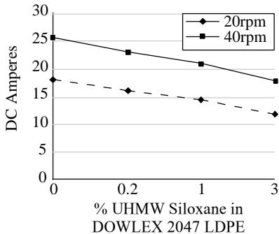
Figure 4: Amperage effect in single screw extrusion.
