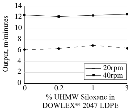
Figure 3: Output effect in single screw extrusion.
